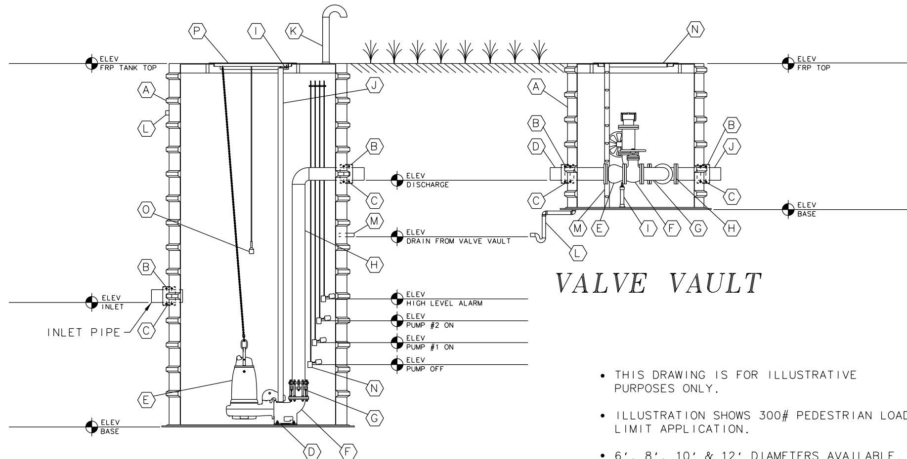
WET WELL
