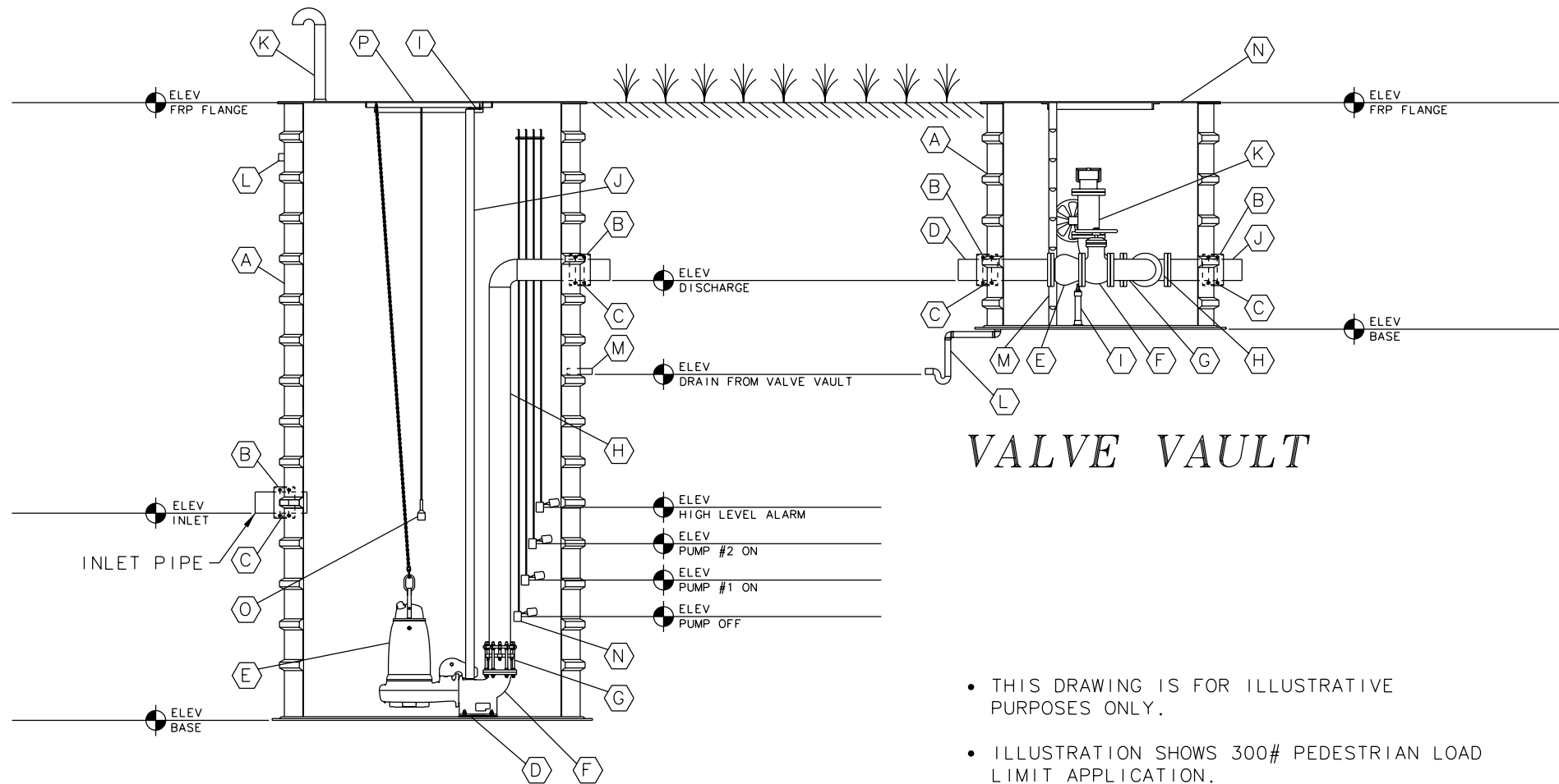
WET WELL
