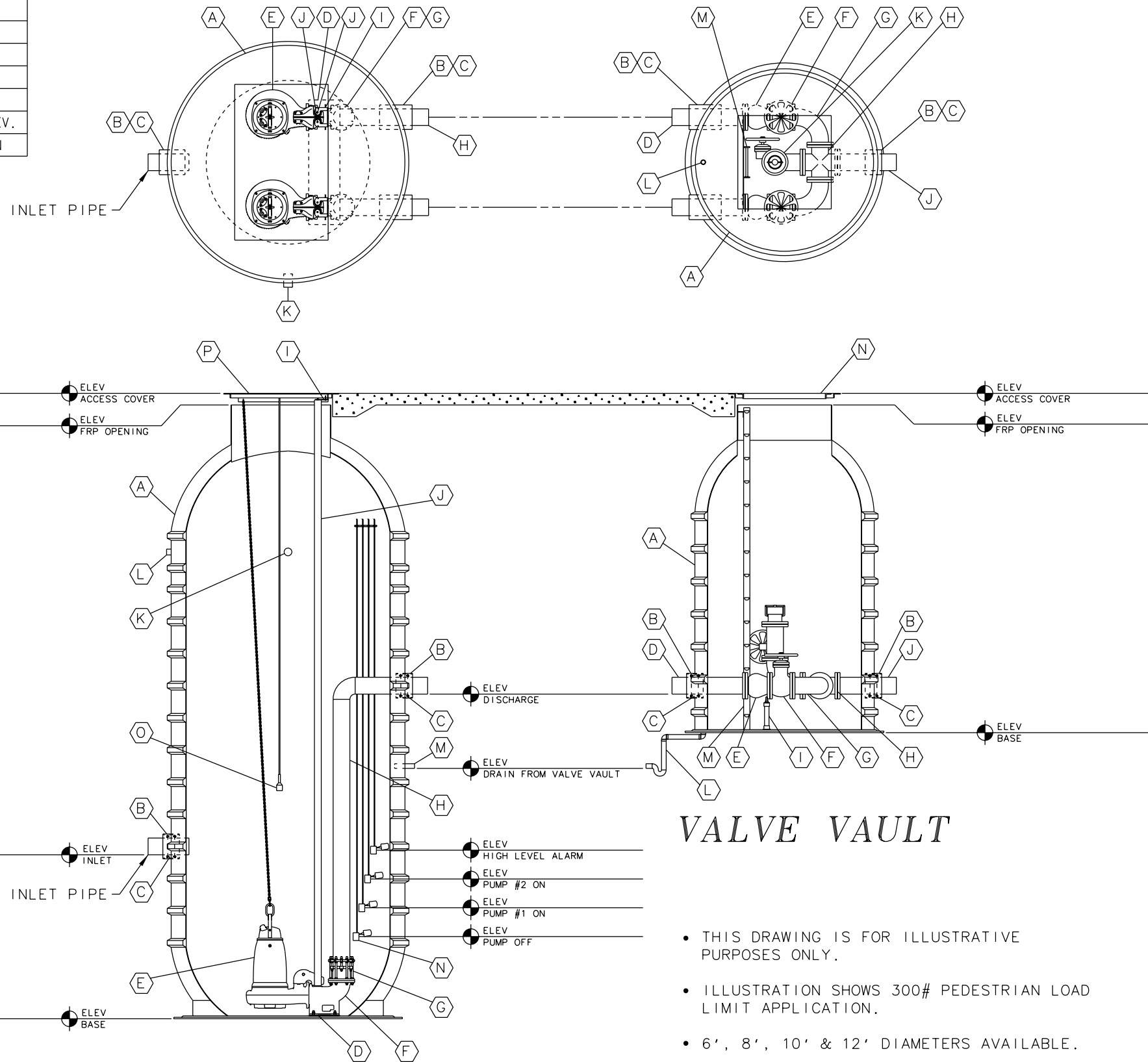
WET WELL
