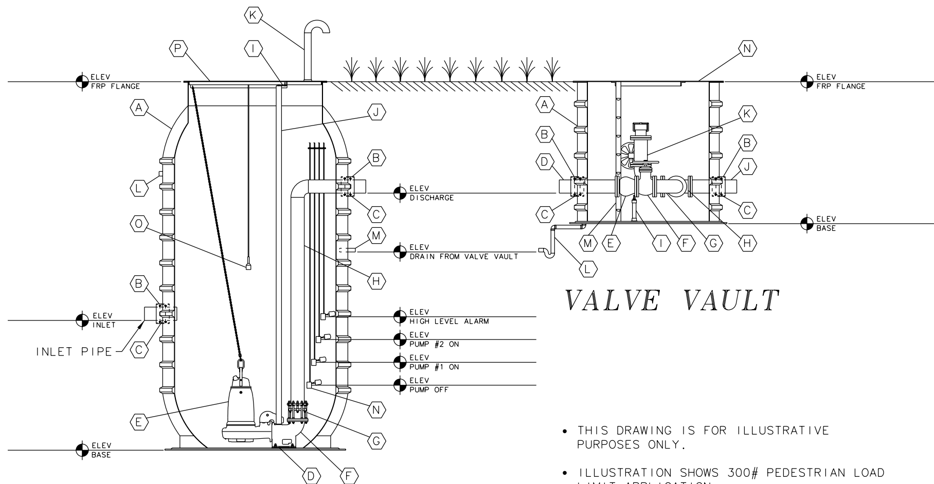
WET WELL
