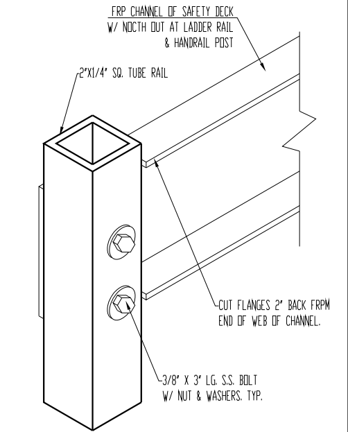
CHANNEL NOTCH DETAIL
