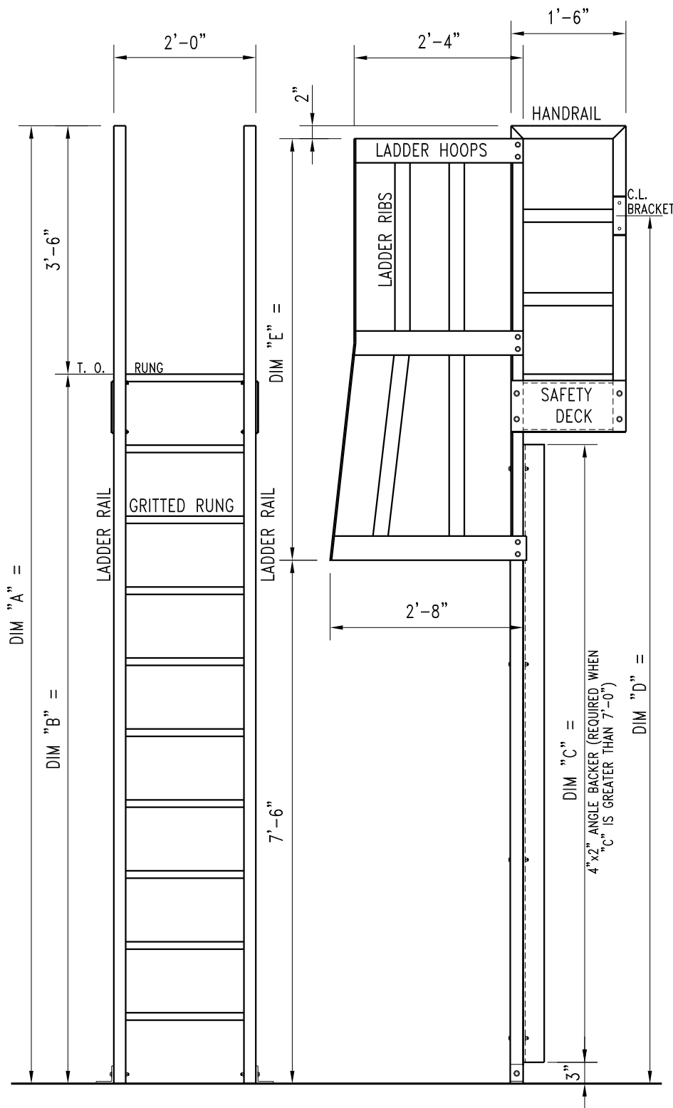
FRP LADDER W/ SAFETY CAGE & DECK
