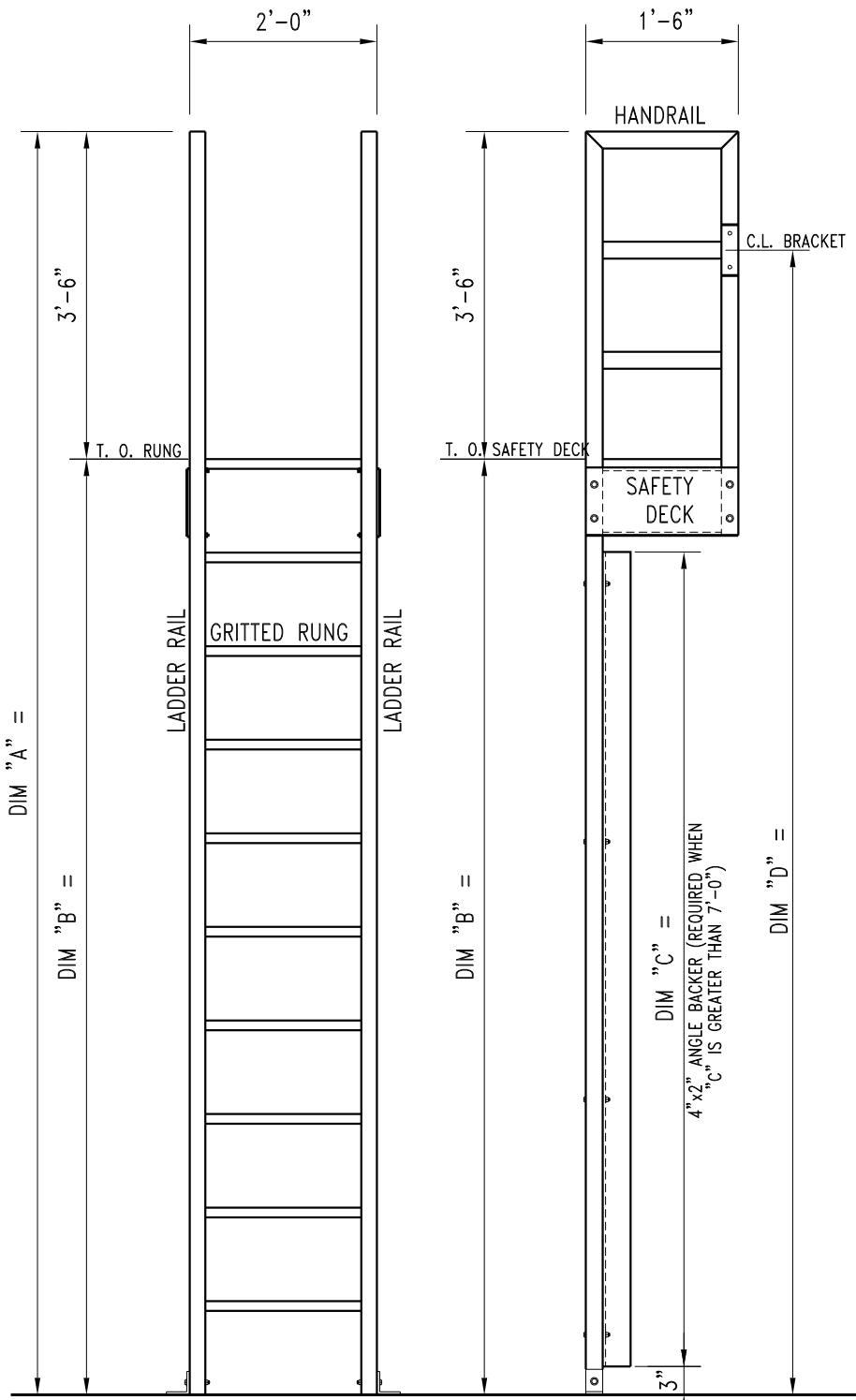
FRP LADDER W/ OPERATOR SAFETY DECK
